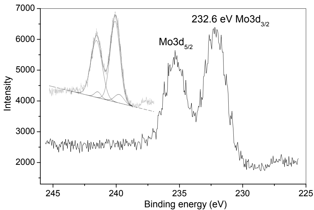
S-Figure 1. XPS spectrum of compound 2.
