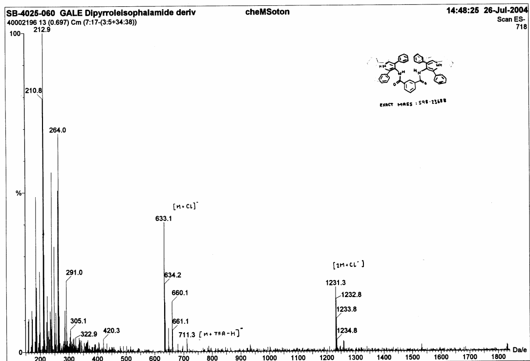
Figure S3 ESMS – of compound 2.
