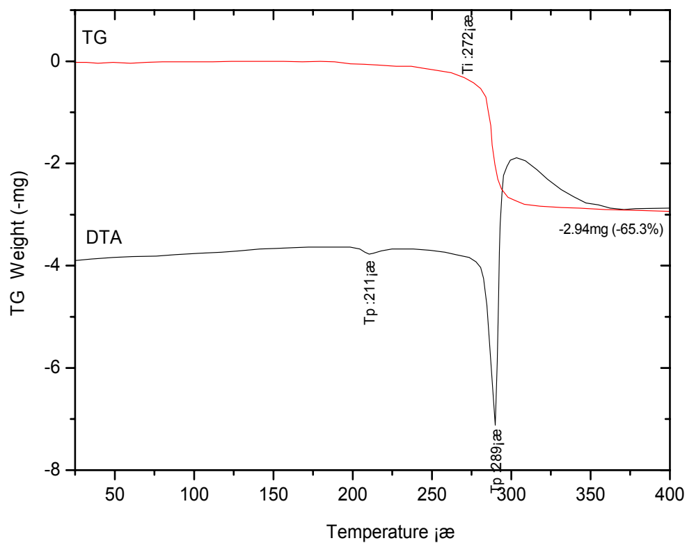
Fig. S6. TG-DTA for 6.
