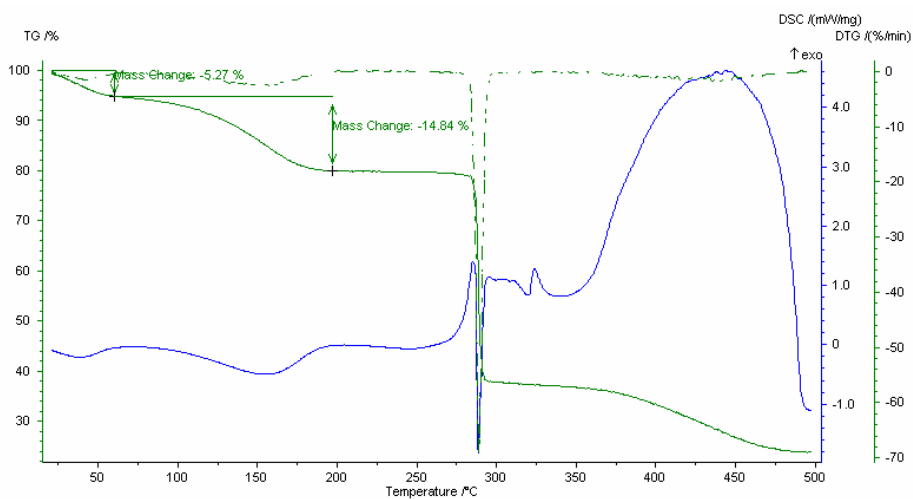
Figure S5 TGA and DSC of \text{Cu}_2(\text{BPDC})_2(\text{BIPY}) from EtOH.
