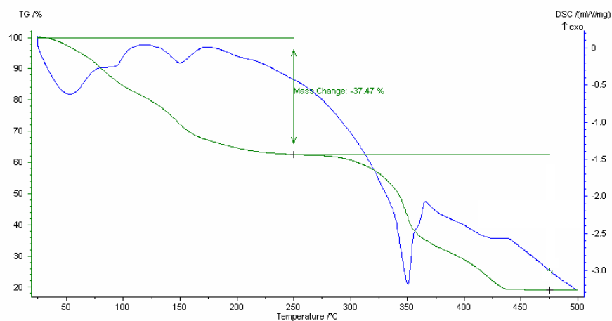
Figure S4 – TGA and DSC of \text{Cu}_2(\text{BPDC})_2(\text{BIPY}) from DMSO.
