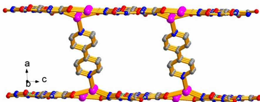
Figure S2. View of the bilayer in 1 along b axis.
