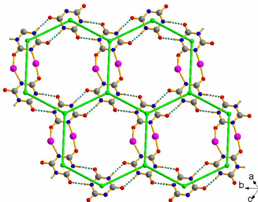
Figure S1. The honeycomb layer in 1.
