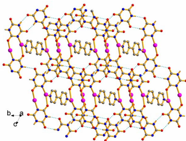
Figure S3. View of the bilayer in 1 along a axis.
