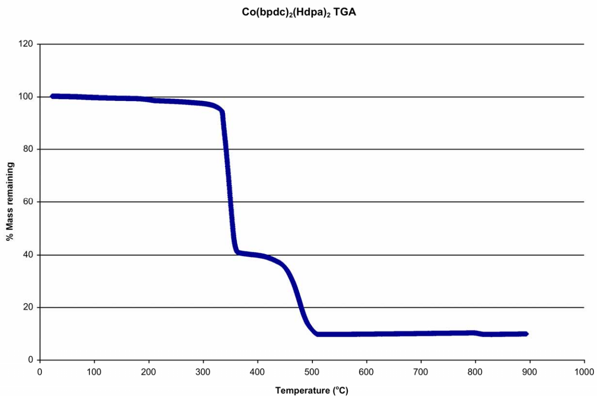
Figure S1. TGA trace for complex 1 .
