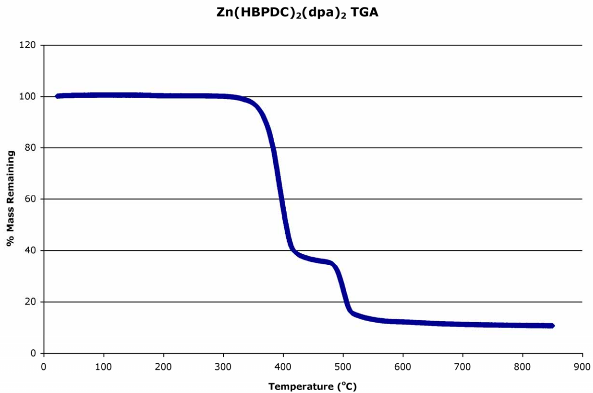
Figure S3. TGA trace for complex 2 .
