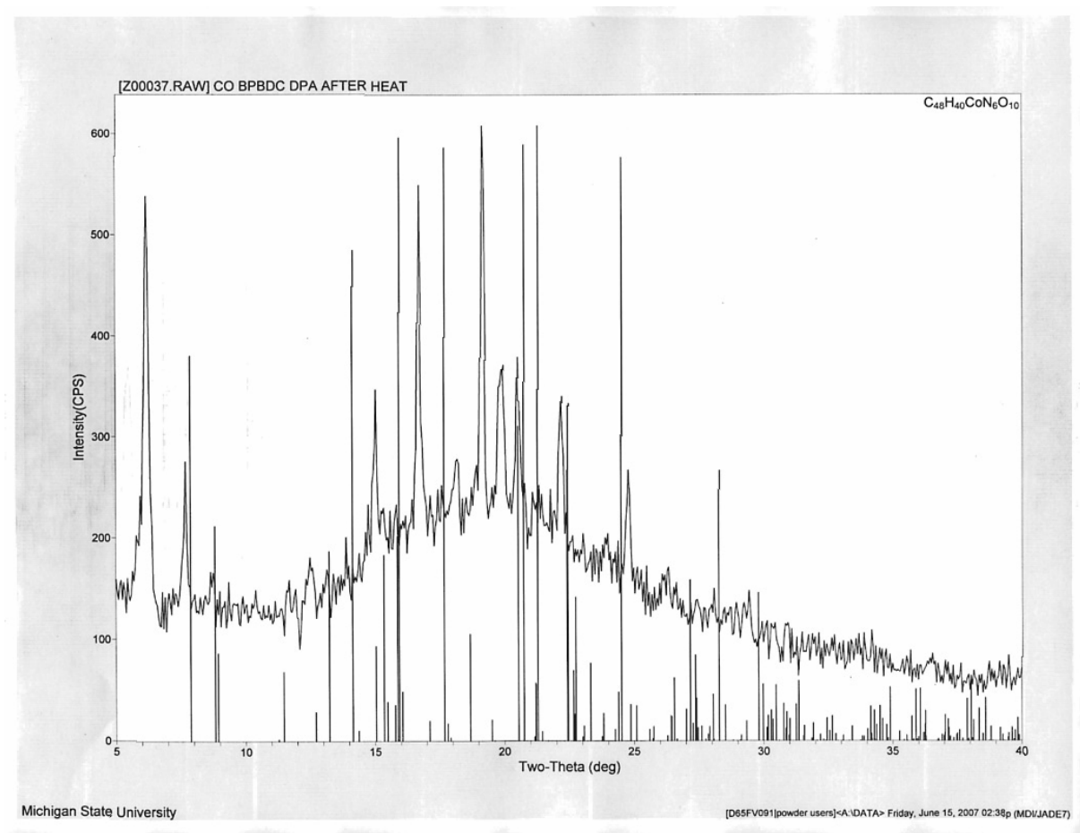
Figure S2. Powder XRD of a sample of 1 that had been thermolyzed in air at 180 °C. The thin black lines correspond to the calculated powder pattern of 1 .
