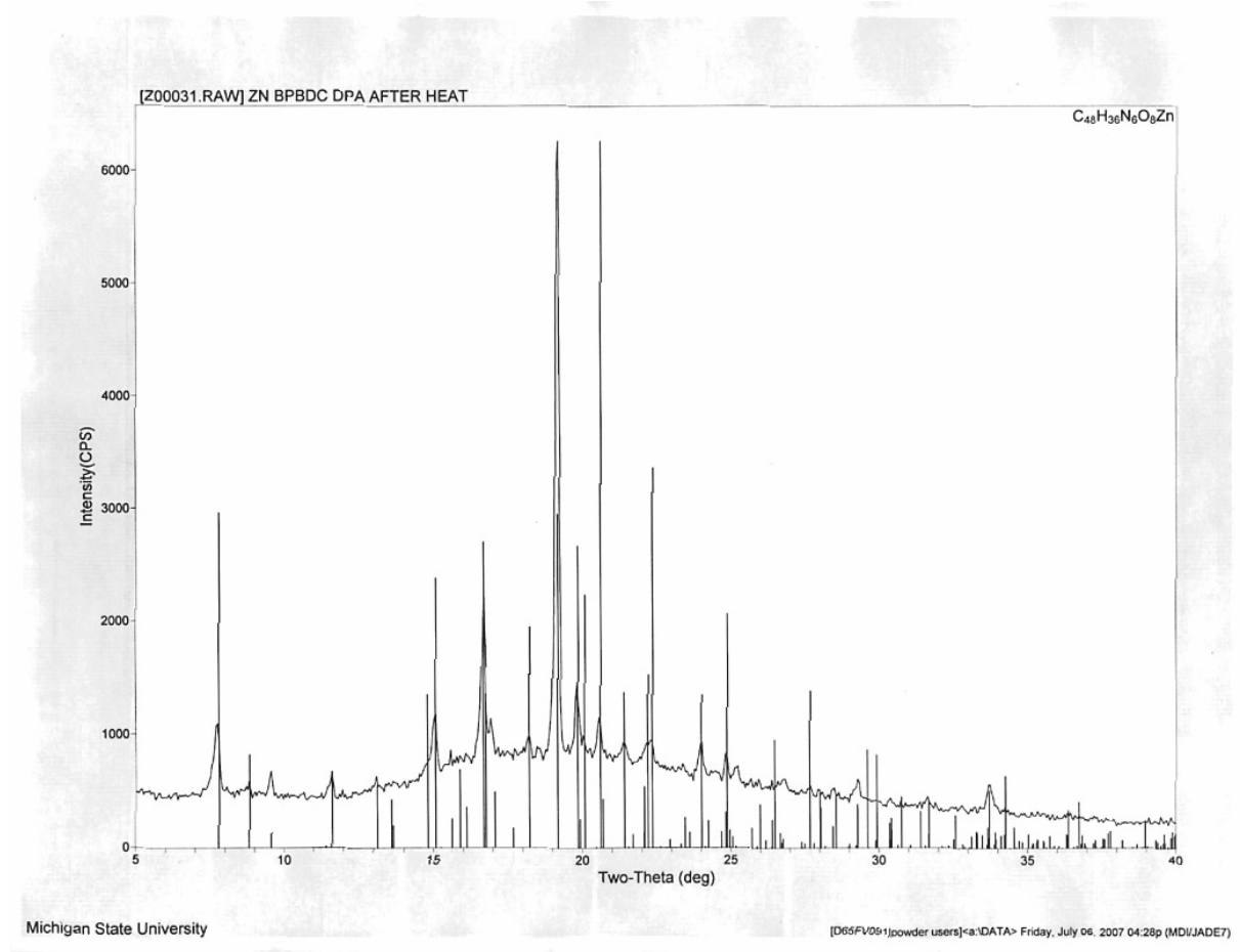
Figure 4. Powder XRD of a sample of 2 that had been thermolyzed in air at 180 °C. The thin black lines correspond to the calculated powder pattern of 2 .
