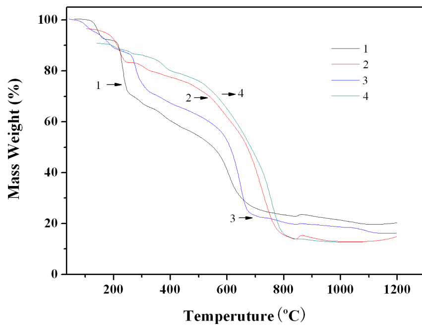
S-2. TGA diagrams of compounds 1–4.
