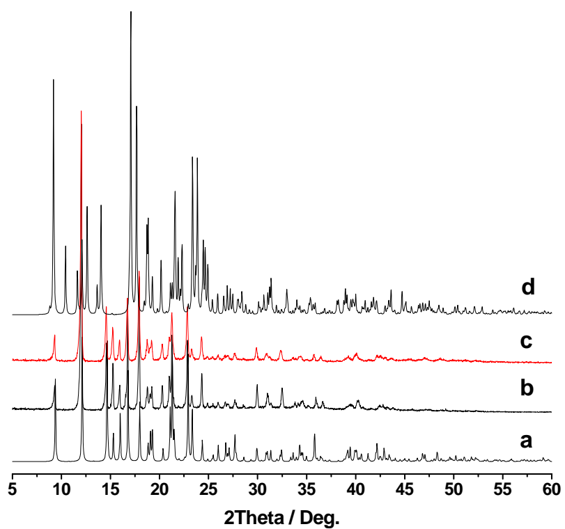
Fig. S2 PXRD patterns of: (a) simulated of 1 , (b) as made of 1 , (c) dehydrated 1 and (d) simulated of 2 .
