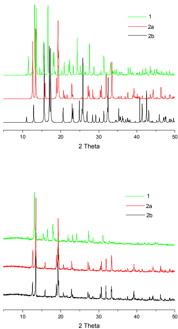
Figure S2. The patterns of XRPD of 1 , 2a and 2b , simulated patterns (top) and diffractive patterns (bottom).
