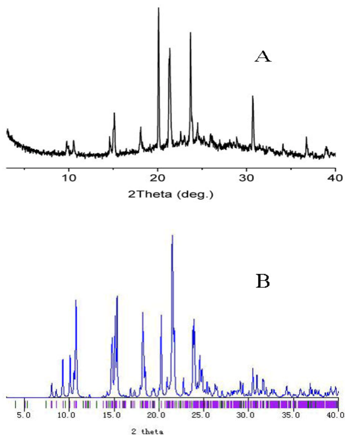
Fig. S4 The measured (A) and simulated (B) XRPD patterns for 1
