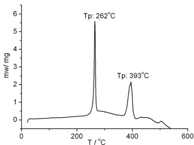
Fig. S3. The DSC curve of compound 1 .
