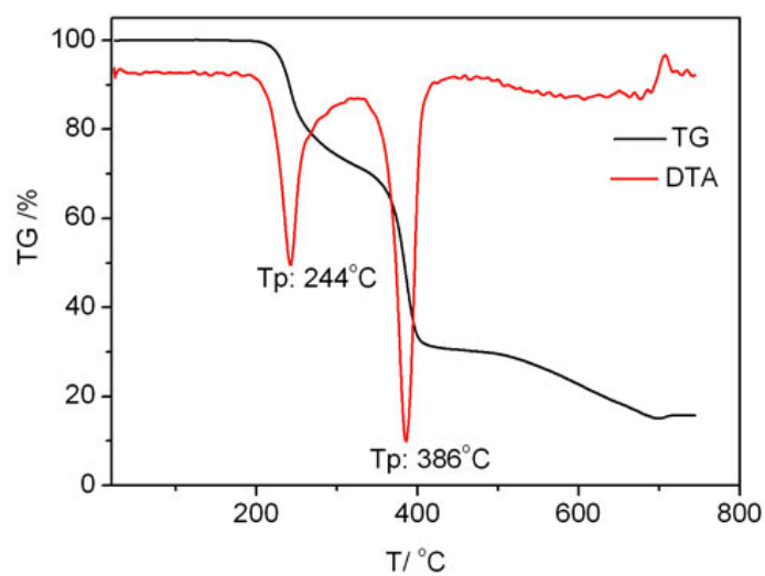
Fig.S2. The TGA-DTA curve of compound 1 .
