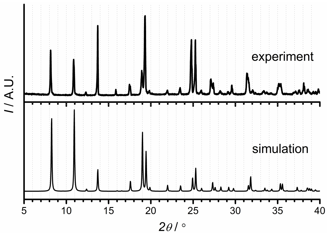
Figure S2. X-ray powder diffraction patterns for 1 .
