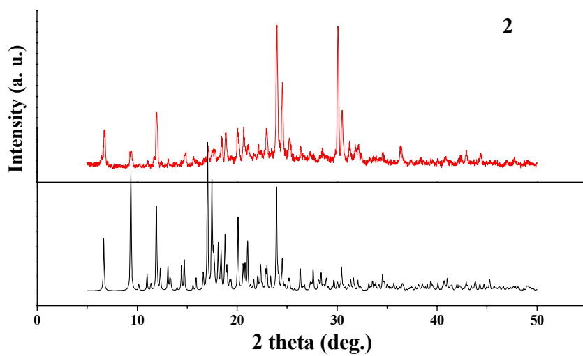
Figure S2. Simulated (black) and experimental (red) XRD spectra for 2
