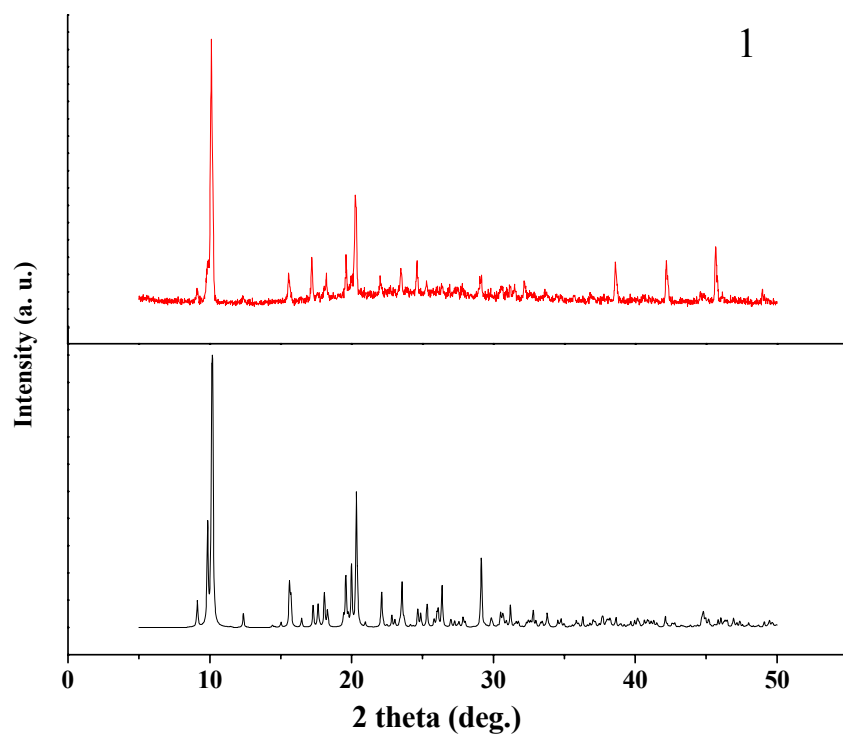
Figure S1. Simulated (black) and experimental (red) XRD spectra for 1
