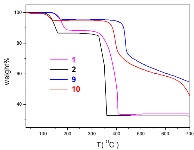
Figure S1. The TGA curves of compounds 1, 2, 9 and 10.
