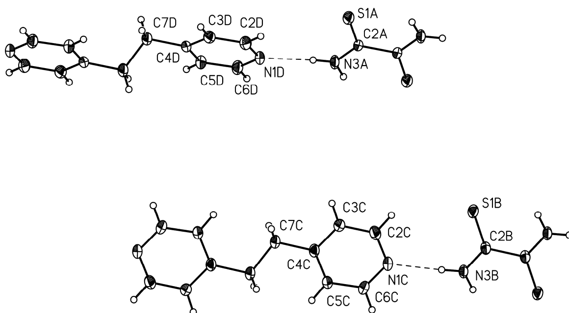
Fig. 2s Ortep drawing of dtox·2 with displacement ellipsoids shown at the 50% probability level
