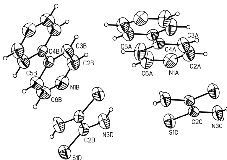
Fig. 1s Ortep drawing of dtox·1 with displacement ellipsoids shown at the 50% probability level
