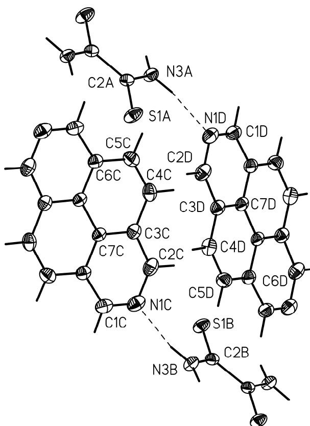
Fig. 3s Ortep drawing of dtox·3 with displacement ellipsoids shown at the 50% probability level
