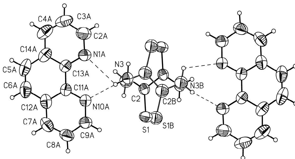
Fig. 7s Ortep drawing of dtox·6 with displacement ellipsoids shown at the 50% probability level
