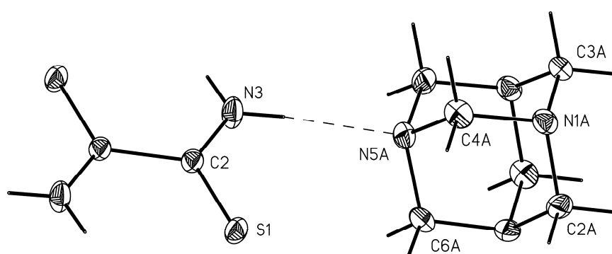
Fig. 6s Ortep drawing of dtox·5 with displacement ellipsoids shown at the 50% probability level
