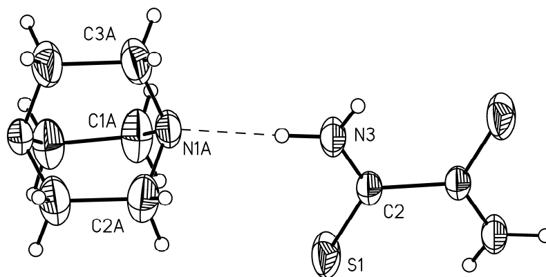
Fig. 3s Ortep drawing of dtox·3 with displacement ellipsoids shown at the 50% probability level
