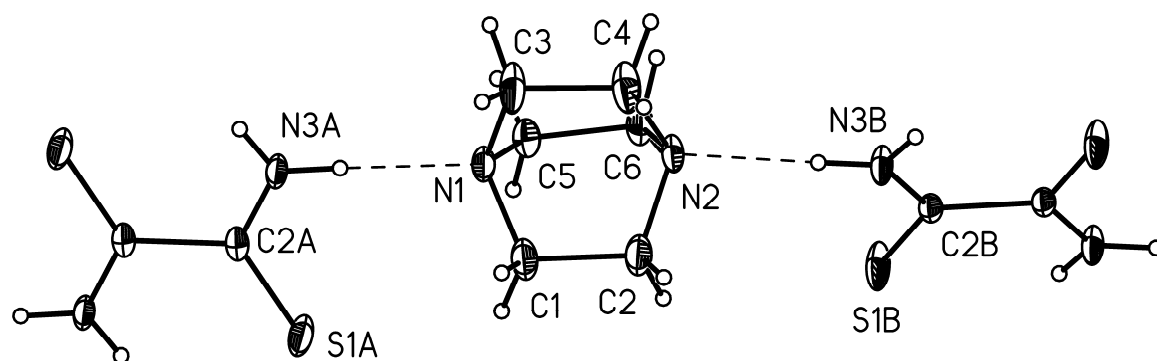
Fig. 5s Ortep drawing of dtox·4lt with displacement ellipsoids shown at the 50% probability level
