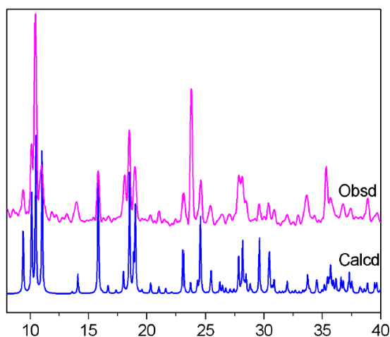
Figure S2. Power X-ray diffraction pattern of the as-synthesized sample of compound 2 and that calculated from single-crystal data.
