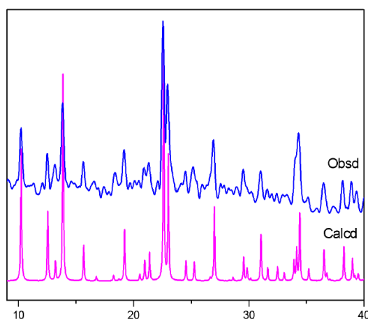
Figure S1. Power X-ray diffraction pattern of the as-synthesized sample of compound 1 and that calculated from single-crystal data.
