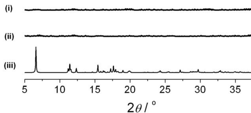
Fig. S2 XRD patterns of (i) the resulted samples at the first water-loss step of TGA; (ii) the resulted samples at the second water-loss step of TGA and (iii) rehydrated samples.
