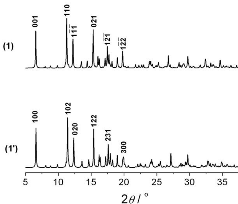
Fig. S3 The comparison of calculated XRD patterns between 1 and 1' .
