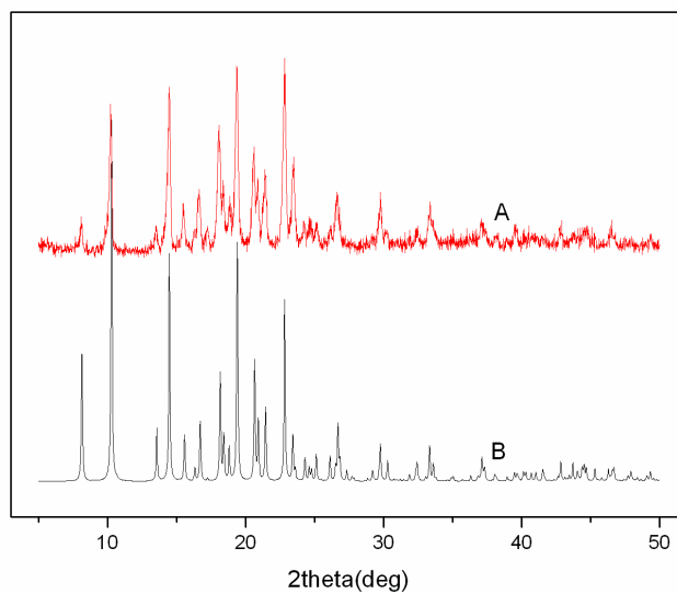
Figure S1. (A) Experimental PXRD pattern of a fresh bulk sample of 1 ; (B) simulated PXRD pattern calculated from the single crystal XRD data for 1 .
