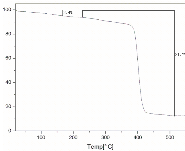
Figure S2 Thermogravimetric analysis curve of 1 .
