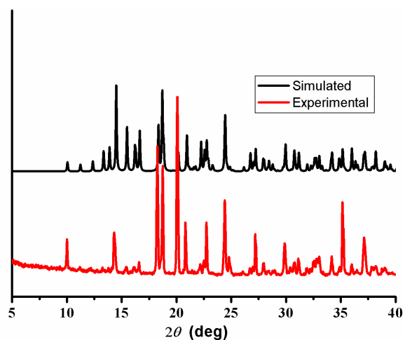
Fig. S1. XRPD for 2
