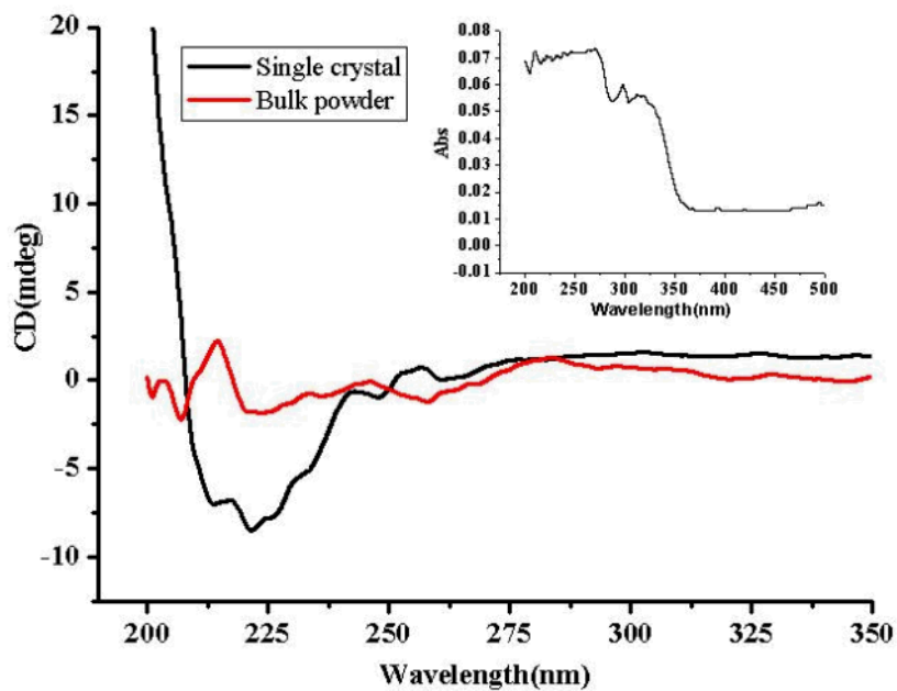
Fig. S3. Solid state CD spectra of 2 (inset: solid-state UV absorption spectrum of 2)
