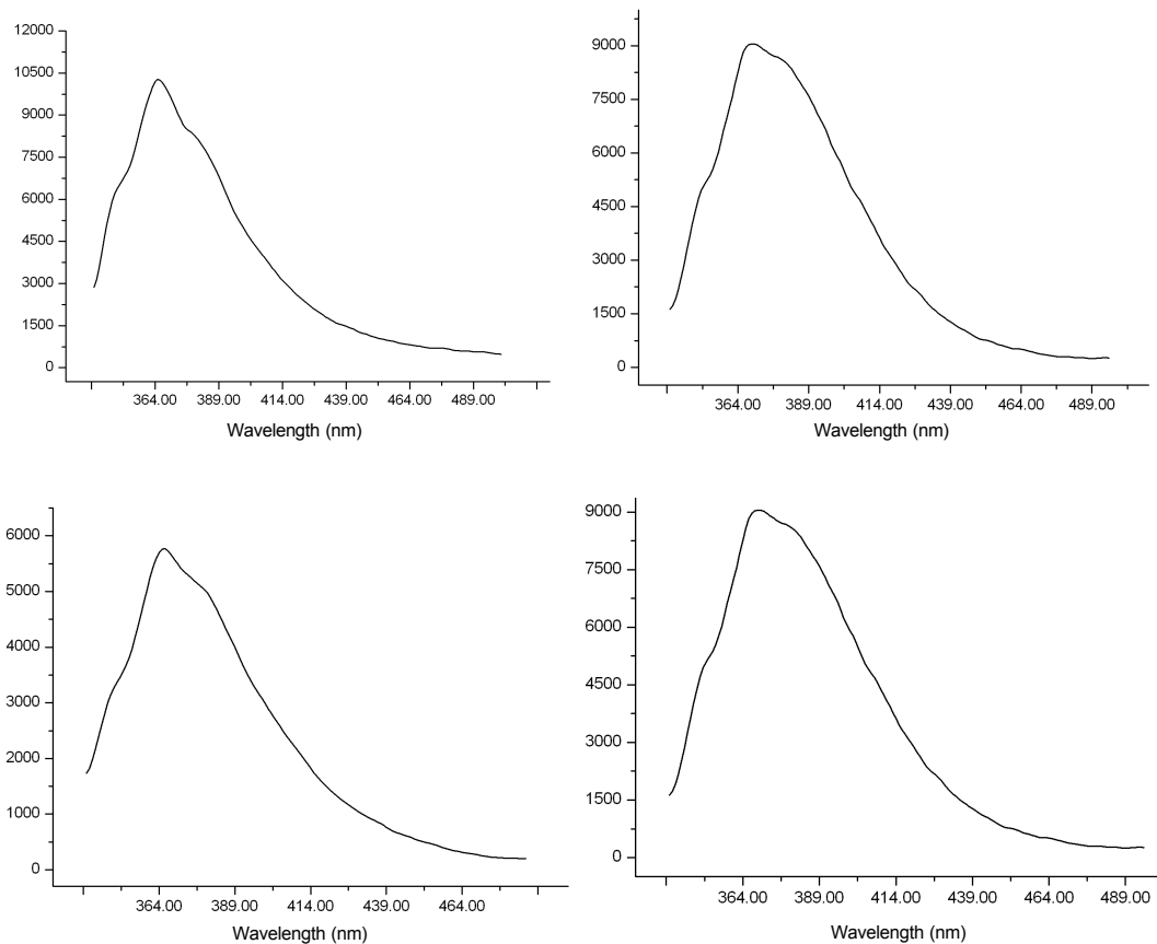
Figure S1. The solid state emission spectra of 1-8 .
