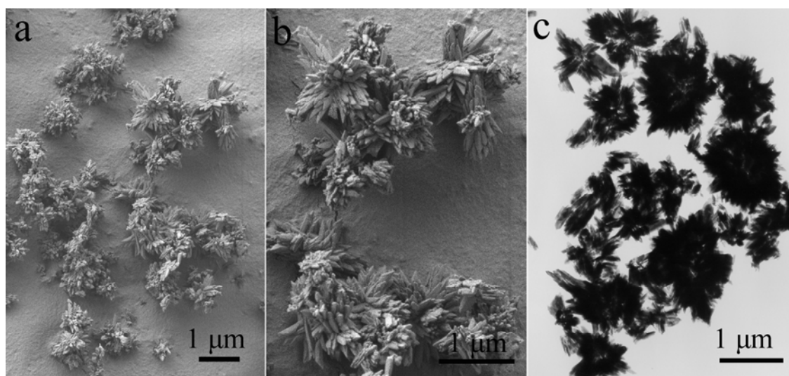
Supporting information, Fig. S1 SEM and TEM images of \text{YW}_2\text{O}_6(\text{OH})_3\text{:Eu} obtained at pH=4.
