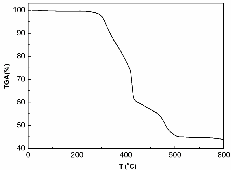
Fig. S1. The TG analysis for compound 1.
