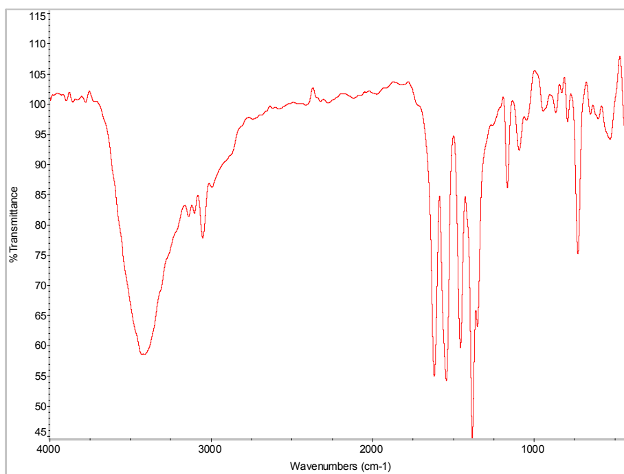
Fig. S4. IR spectra for compound 2.
