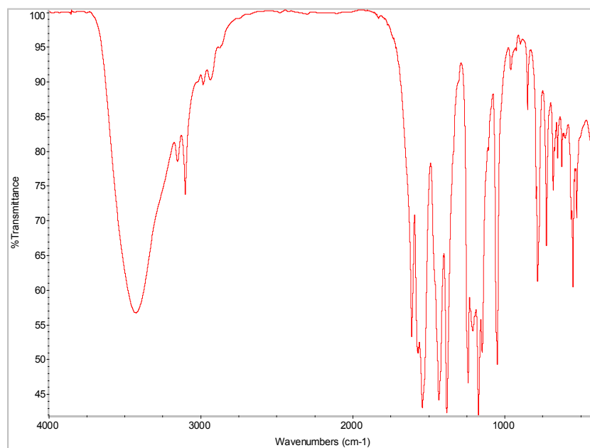
Fig. S3. IR spectra for compound 1.
