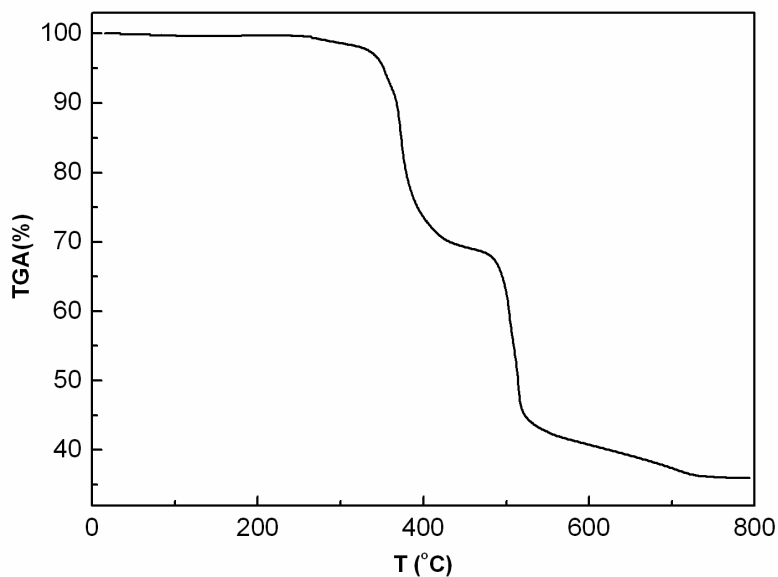
Fig. S2. The TG analysis for compound 2.
