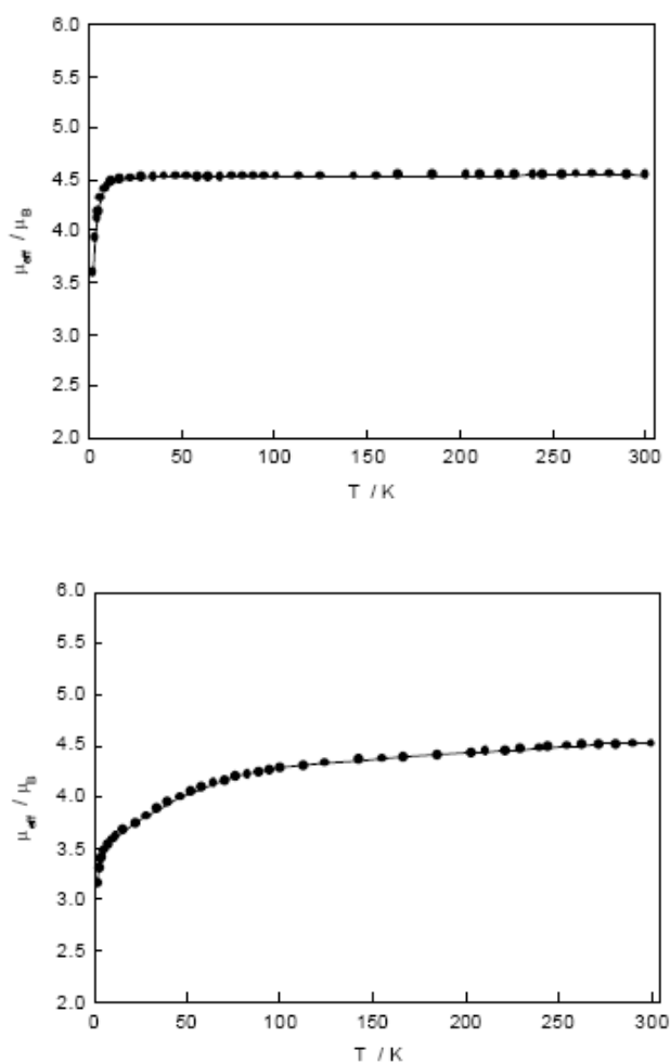
Figure S1: Plots of \mu_{\text{eff}} vs temperature per \text{M}^{\text{II}} in an applied field of 1 T for 2\text{Fe} (top) and 2\text{Co} (bottom). The solid lines merely join the dots.
