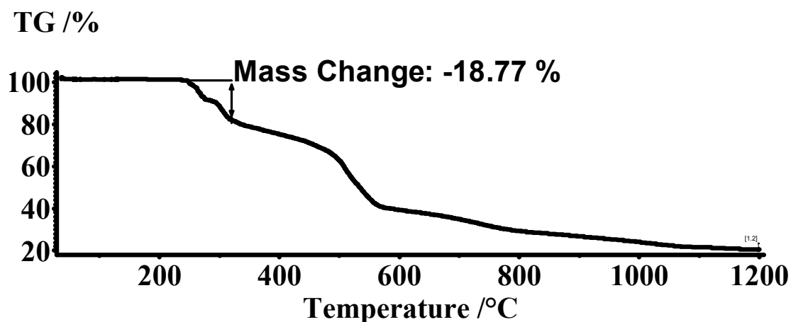
Fig. S1 The TGA curve of compound 1 under nitrogen atmosphere.
