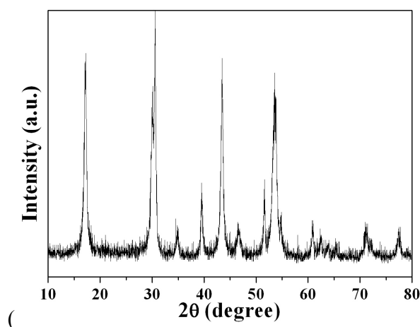
Fig. S1 XRD pattern of \text{Na}(\text{Y}_{1.5}\text{Na}_{0.5})\text{F}_6 nanospindles prepared at room temperature for 20 h.
