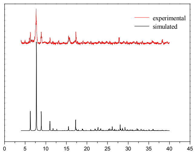
Fig. s7 the experimental and simulated XRD pattern for 2 .
