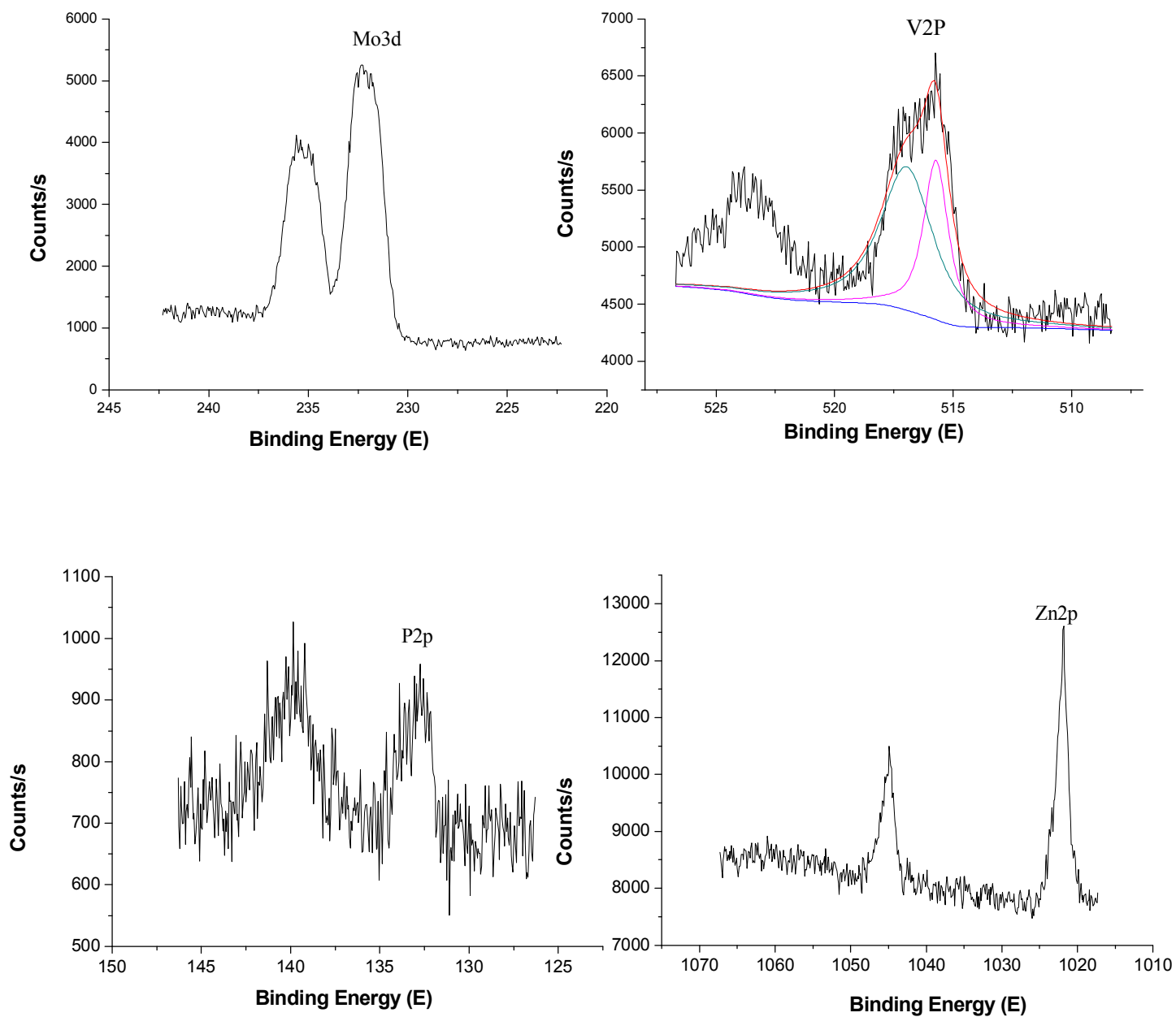
Fig. s3 The XPS spectra for compound 3.
