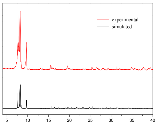
Fig. s10 the experimental and simulated XRD pattern for 5 .
