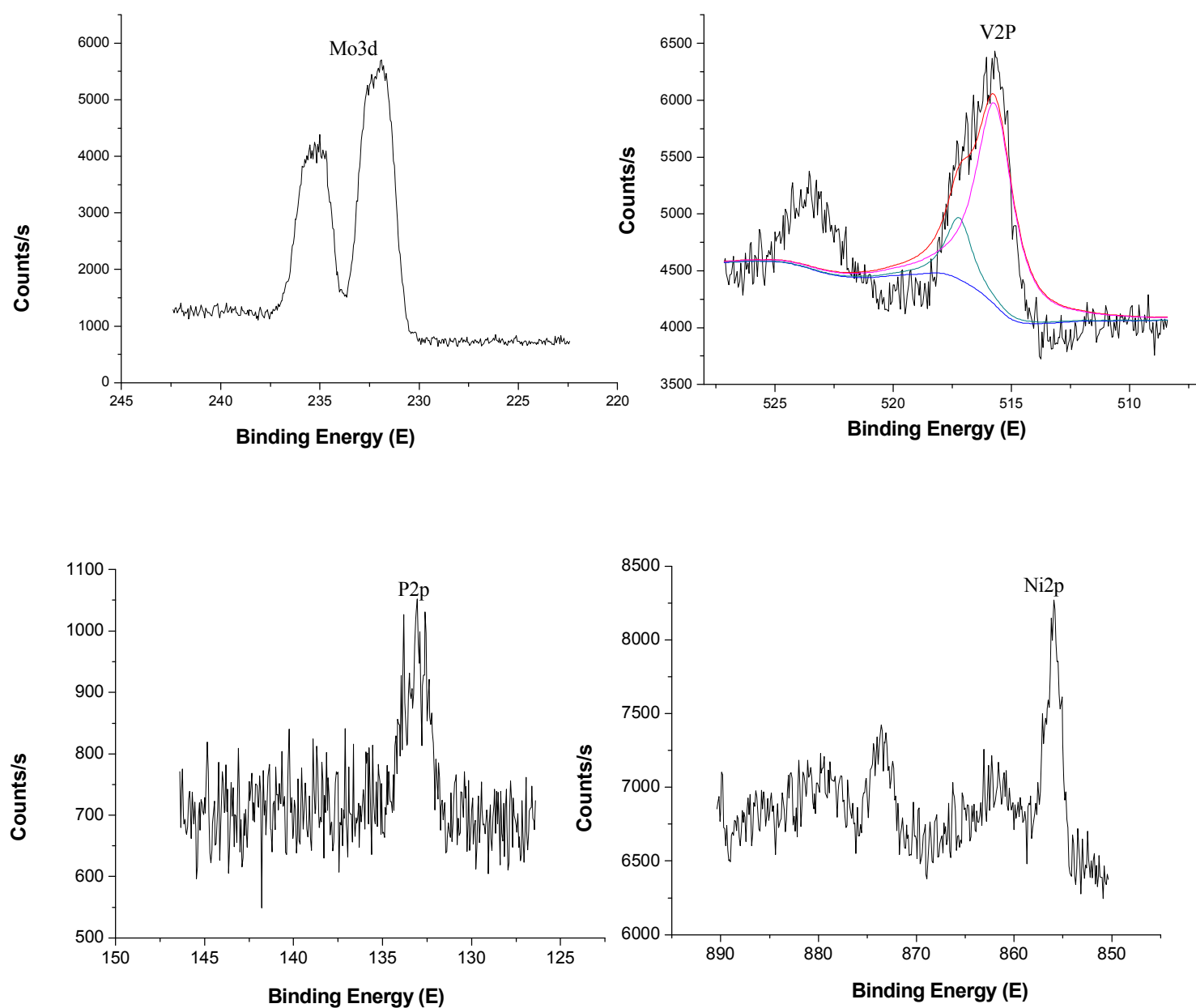
Fig. s2 The XPS spectra for compound 2.
