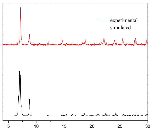
Fig. s9 the experimental and simulated XRD pattern for 4.
