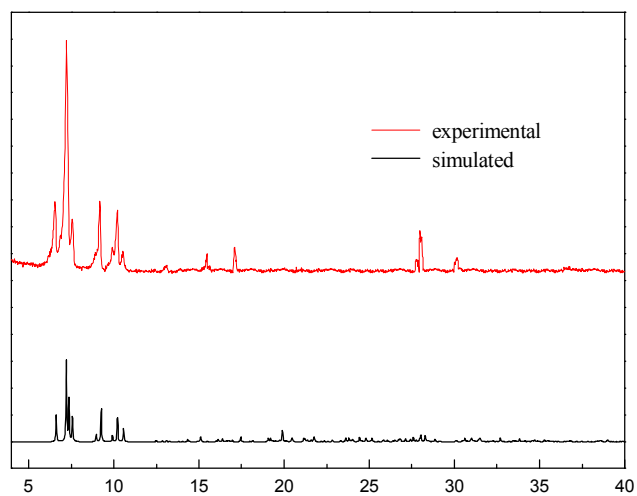
Fig. s8 the experimental and simulated XRD pattern for 3 .
