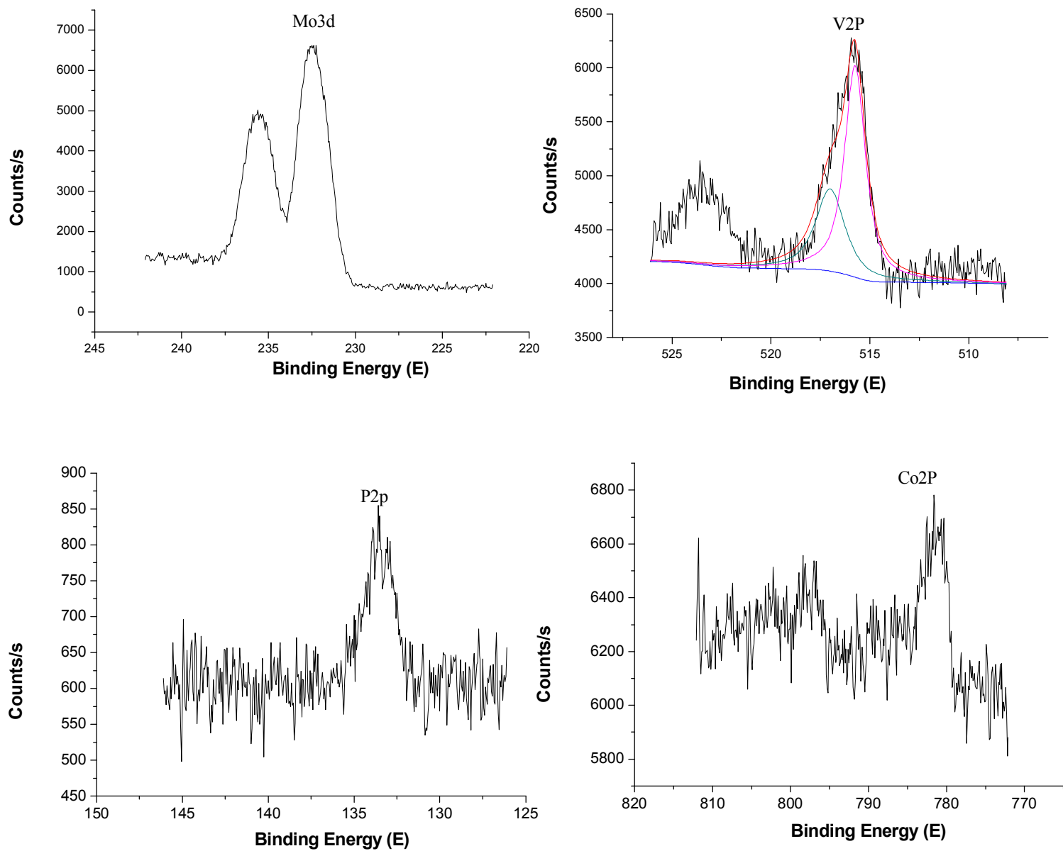
Fig. s5 The XPS spectra for compound 5.
