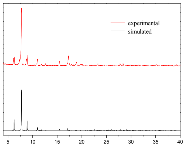
Fig. s6 the experimental and simulated XRD pattern for 1 .
