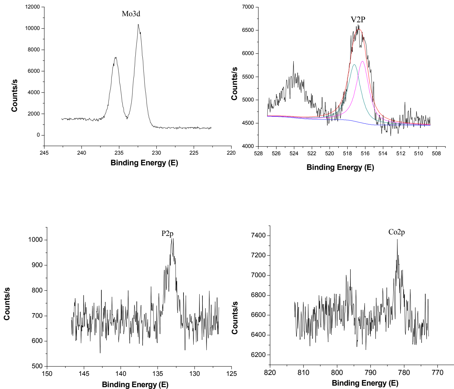
Fig. S4 The XPS spectra for compound 4.
