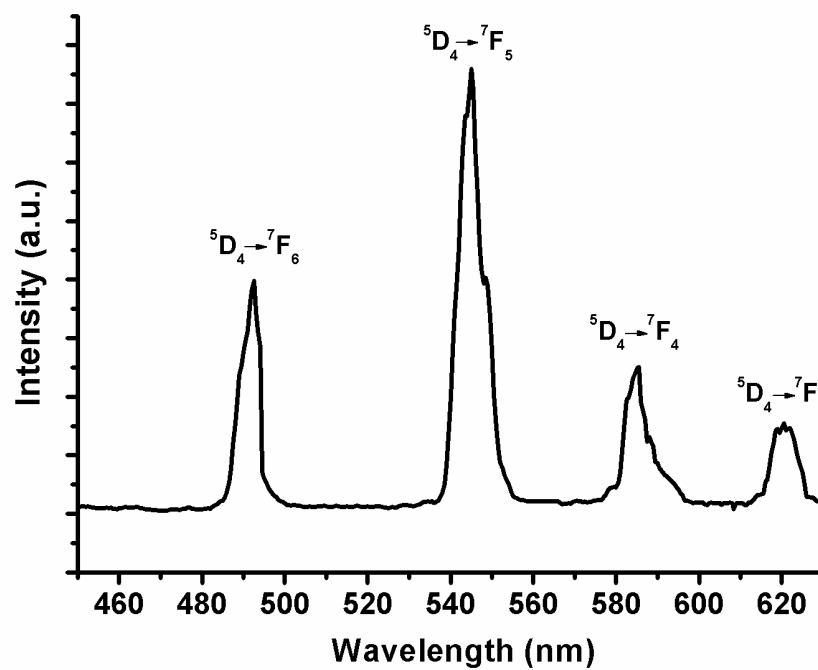
Fig. S3. Solid-state emission spectrum of 1a at room temperature.
