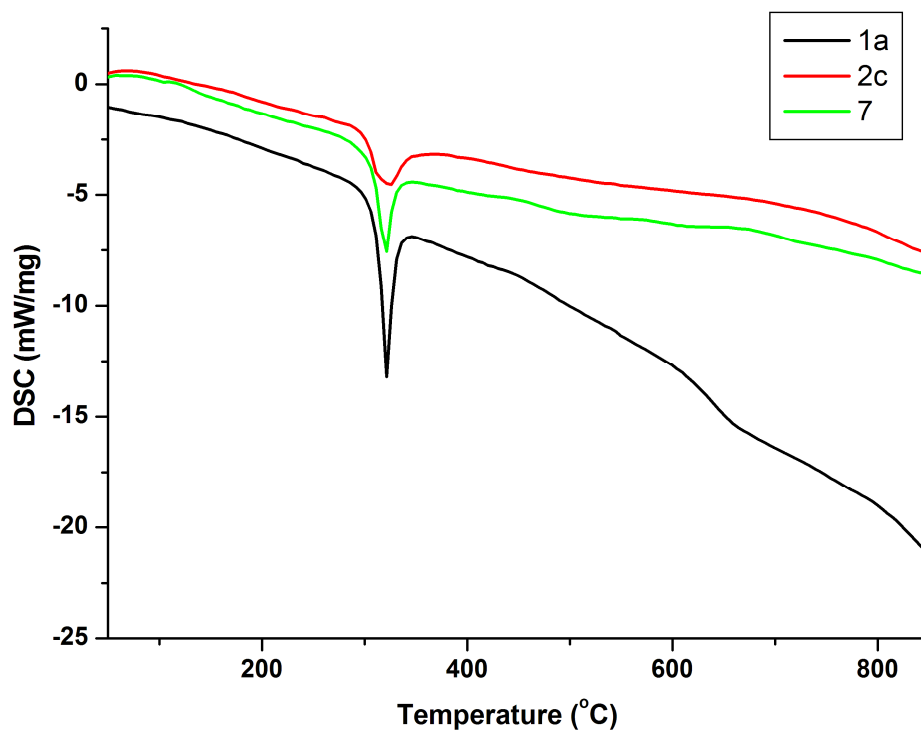
Fig. S2. DSC traces of complexes 1a, 2c and 7 involving perchlorate ions.
