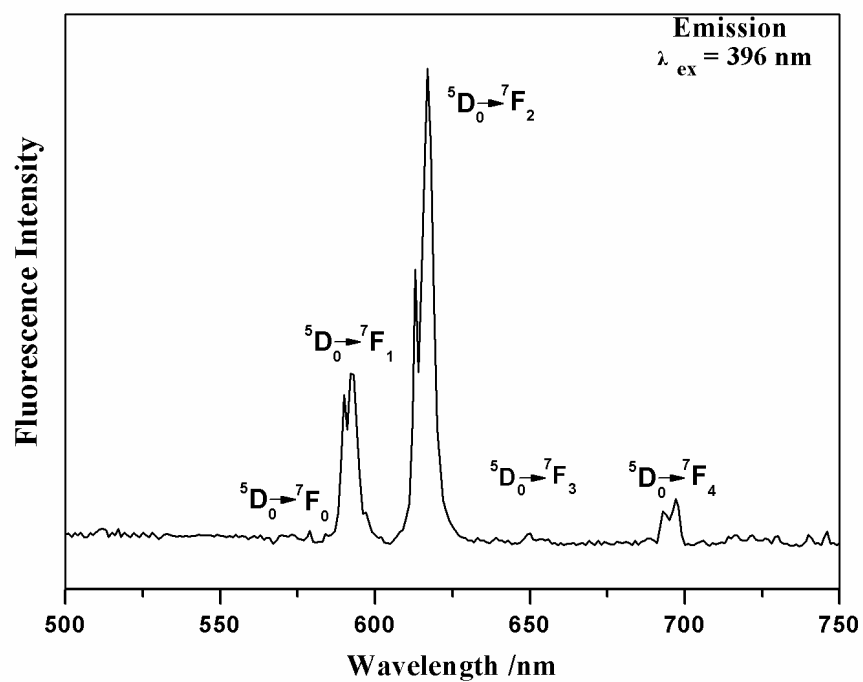
Fig. S4. Solid-state emission spectrum of 2b at room temperature.
