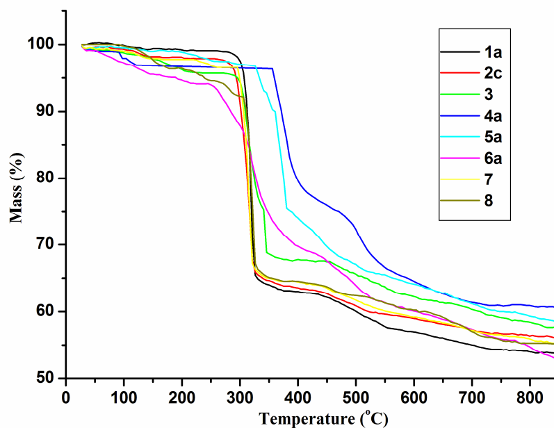
Fig. S1. TGA traces of representative complexes.
