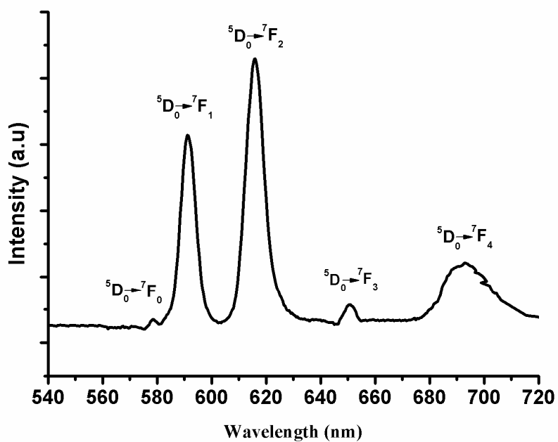
Fig. S5. Solid-state emission spectrum of 8 at room temperature.
