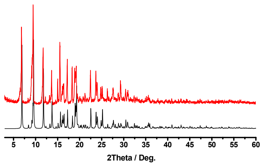
Fig. S2 PXRD patterns of 2 : red represents as made and black represent simulated one from crystal data.
