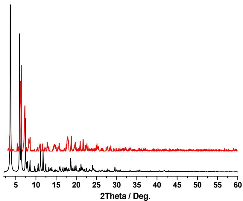
Fig. S1 PXRD patterns of 1 : red represents as made and black represent simulated one from crystal data.
