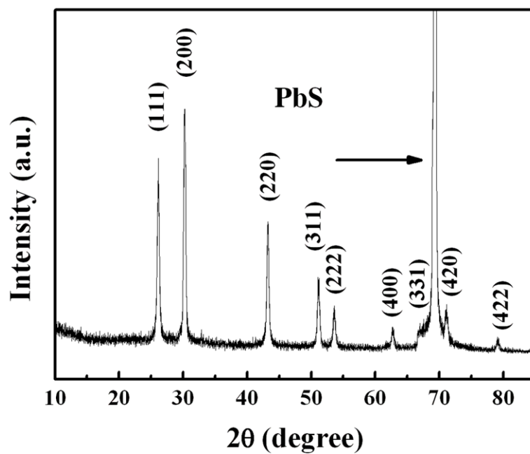
Fig. S2 XRD pattern of the cubic PbS nanocrystals shown in Figure 6 c. Arrow indicated peak was from Si wafer.
