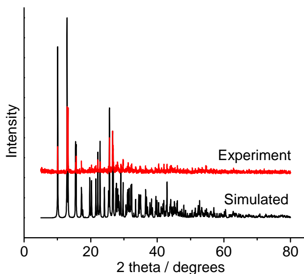
Fig. S1 Simulated and experimental XRD powder patterns for compound 1 .
