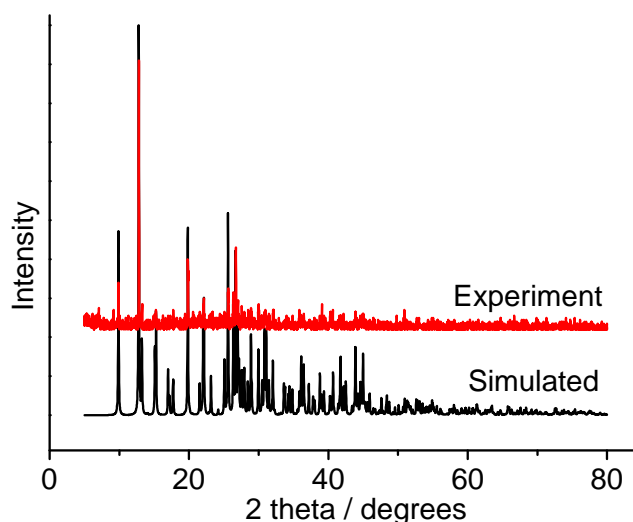
Fig. S2 Simulated and experimental XRD powder patterns for compound 2 .
