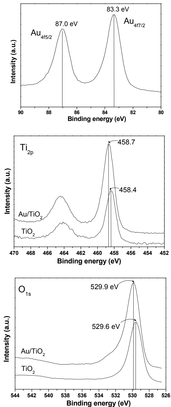
Fig. S1 XPS spectra of Au4f, Ti2p and O1s of the pure and gold-doped rutile TiO 2 .
