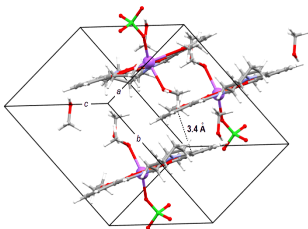
Fig. S1 Assembly of [\text{Cu}\{(R,R)\text{-1}\}\text{Na}(\text{CH}_3\text{OH})(\text{OCIO}_3)] molecules in [\text{Cu}\{(R,R)\text{-1}\}\text{Na}(\text{CH}_3\text{OH})(\text{OCIO}_3)]\cdot\text{CH}_3\text{OH} illustrating \pi -stacking between arene rings.
