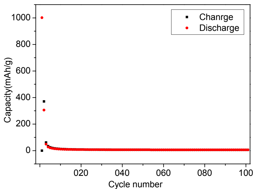
Fig. S1. Diagram of charge-discharge capacity versus cycle numbers.
