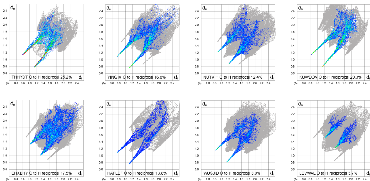
Figure S1 Fingerprint plots for compounds 1-7 resolved into O...H contacts. The full fingerprint appears beneath each decomposed plot in grey.
