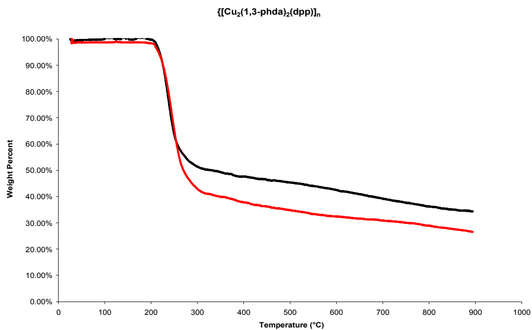
Fig. S1. TGA trace for 1 .
