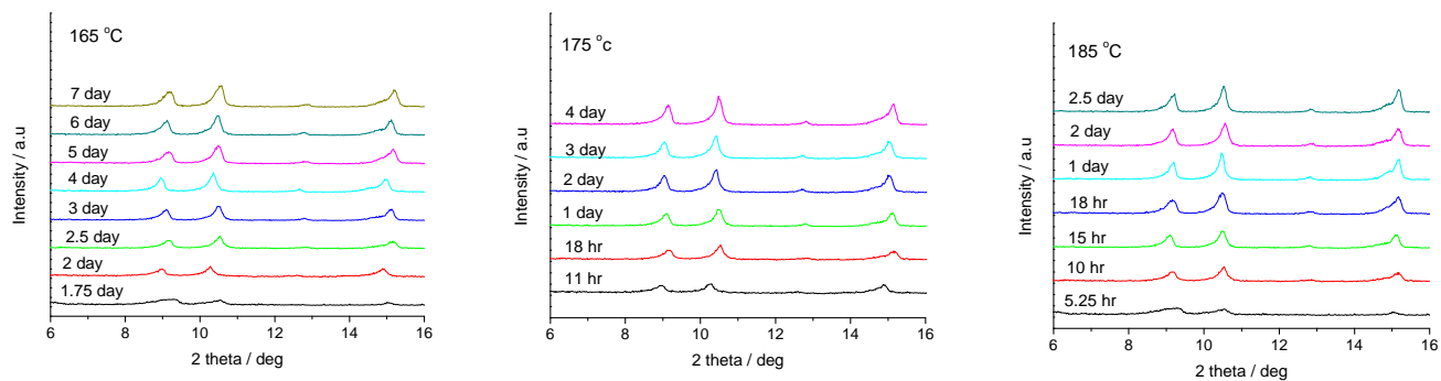
Figure S3. XRD pattern of as-synthesized MIL-53(Cr) at various temperatures and time under conventional electric heating.
