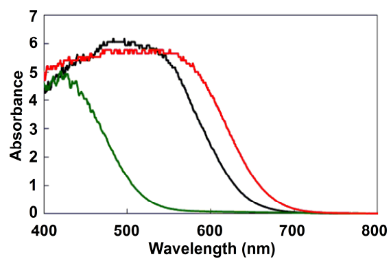
Fig. ESI-1 Optical absorption spectra (the Kubelka-Munk functions derived from the DRS) of CT complexes I (black), II (green), and III (red).
