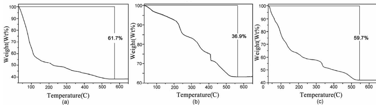
Fig. S2 TGA curves of (a) as-synthesized sample, 1 , (b) guest DMSO-free phase, 1a (c) re-adsorption sample, 1b . The number of guest DMSO molecules per unit cell in the channels is calculated by deduction of the coordinated DMSO molecules and by ligands.
