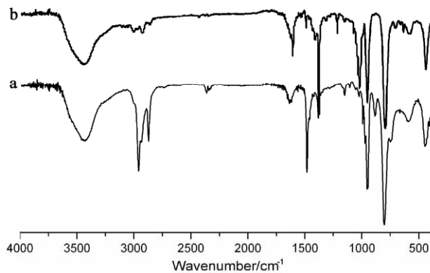
Fig. S1 FT-IR spectra of (a) [(n-C 4 H 9 ) 4 N] 4 [V 2 W 4 O 19 ] and (b) 1 .
