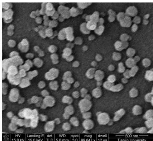
Fig.S1 SEM image of the luminescent hybrid organosilica obtained by reacting \text{Eu}^{3+} ions with TTA-Si under reflux for 4h. The molar ratio of TTA-Si to \text{Eu}^{3+} ions is 1:1
