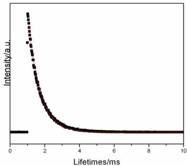
Fig.S2 Decay curve of luminescent organosilica with rectangular-plate morphology squares: experimental data; solid line: fitted according to I = I_0 + A \exp[-(t - t_0)/\tau]
