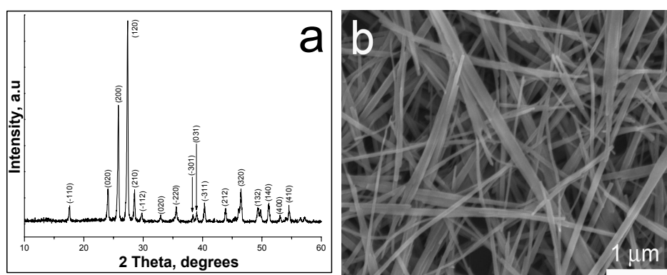
Fig. S1. (a) XRD pattern and (b) SEM images of the as-synthesized \text{SrCrO}_4 nanowires.
