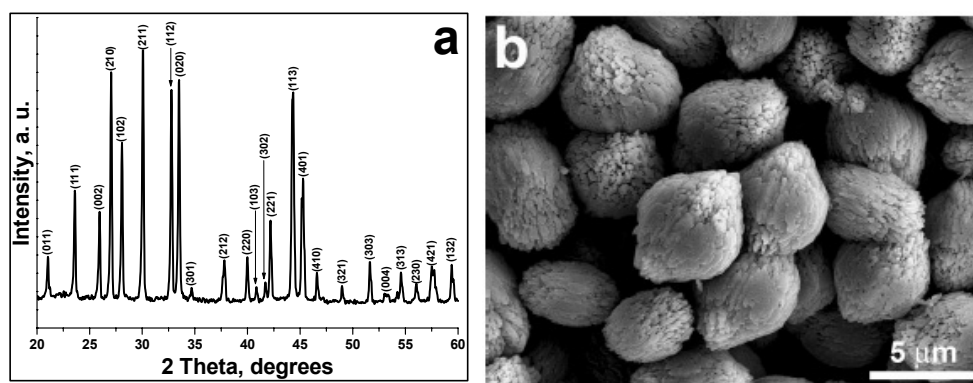
Fig. S2. (a) XRD pattern and (b) SEM image of the \text{SrSO}_4 aggregates obtained by the direct reaction between aqueous \text{SrCl}_2 and \text{Na}_2\text{SO}_4 solutions.
