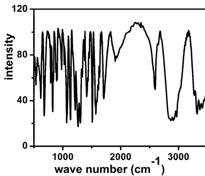
Fig. S2 The IR Spectrum of compound 1 at room temperature I for RT phase.
