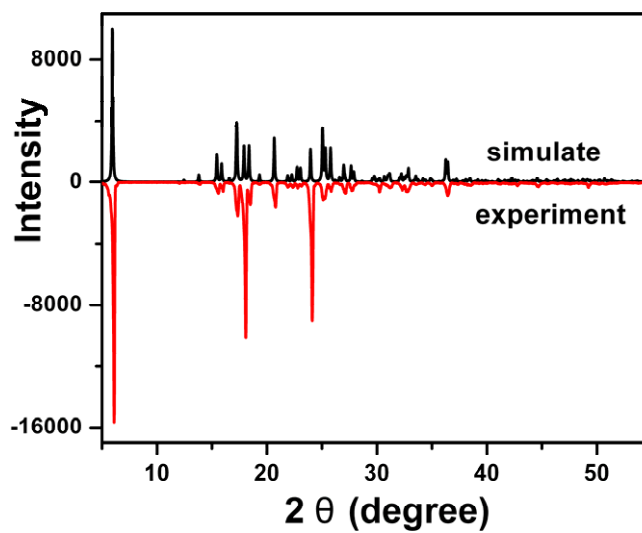
Fig. S1 The experimental and simulated PXRD diagram of compound 1 for RT phase.
