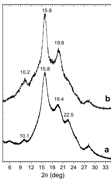
Figure S1. X-ray diffraction patterns, as collected by an automatic powder diffractometer of PS/TEMPO co-crystalline powder samples as obtained by sorption of TEMPO (20% wt/wt chloroform solution) in: (a) amorphous, (b) \epsilon nanoporous form.
