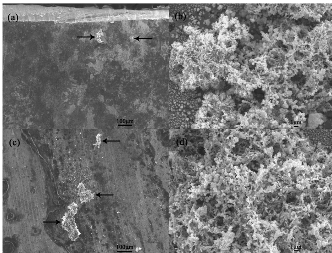
Fig. S1 FE-SEM images with different magnifications of the products obtained in \text{CuCl}_2 aqueous solution ( \text{CuCl}_2 0.007 g, \text{H}_2\text{O} 2.0 mL) at different reaction time. (a) 60 s, low magnification; (b) 60 s, high magnification; (c) 120 s, low magnification; (d) 120 s, high magnification.
