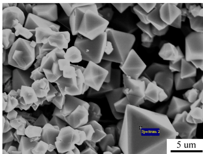
Fig. S2 SEM image of octahedral magnetite
