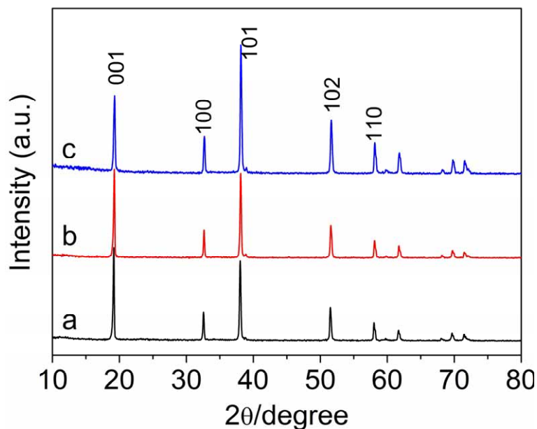
Fig. S1 XRD patterns of \text{Co(OH)}_2 samples synthesized at different time (a) several minutes, (b) 60 min and (c) 240 min.
