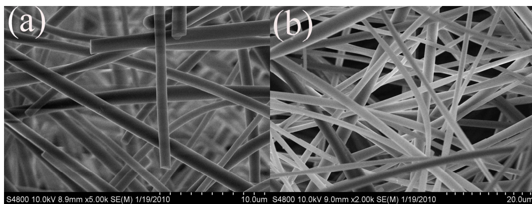
Fig. S1 SEM images of electrospun composite fibers with different addition PVP used 7.5 ml water and 2.5 ml ethanol as solvent (a) 6.00 g; (b) 6.50 g.
