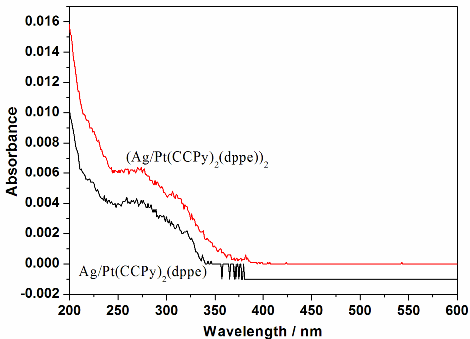
Figure S3. UV-vis spectra of the multilayer film [PEI-(Ag^+/Pt(CCPy)_2(dppe))_n] .
