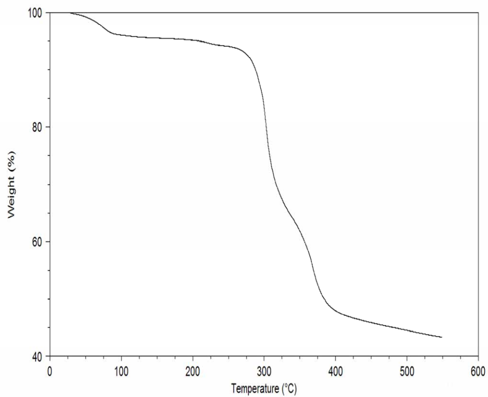
Fig. S3 TGA analysis for 2 .
