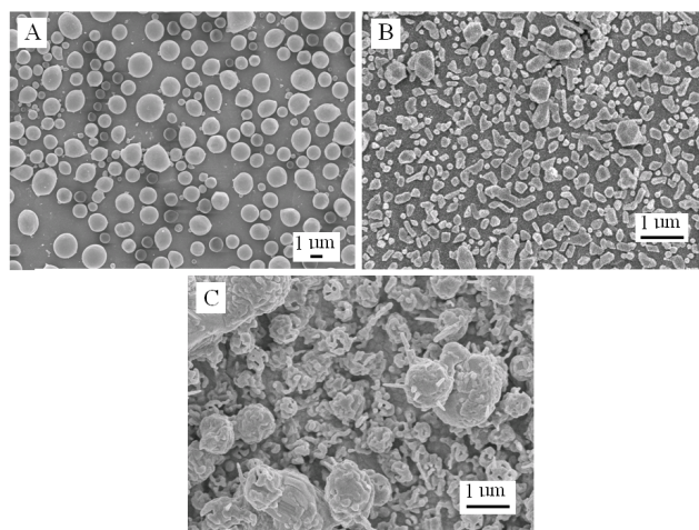
Figure S2 SEM images of the samples synthesized with different oxygen concentrations with continuous \text{O}_2 flow: (A) 0.1%; (B) 1%; (C) 10%. The Bi evaporation temperature is all 800 ^\circ\text{C} .
