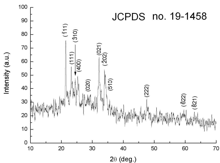
Figure S1 XRD pattern of the precipitates when \text{Na}_2\text{CO}_3 was added.
