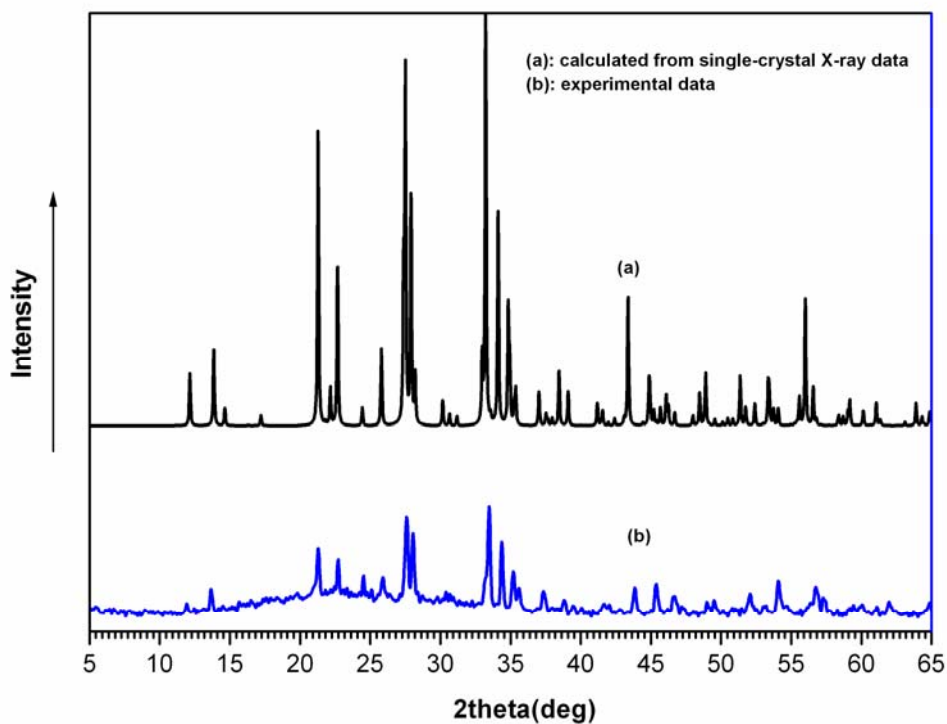
Fig. S3 X-ray powder diffraction pattern for 1.
