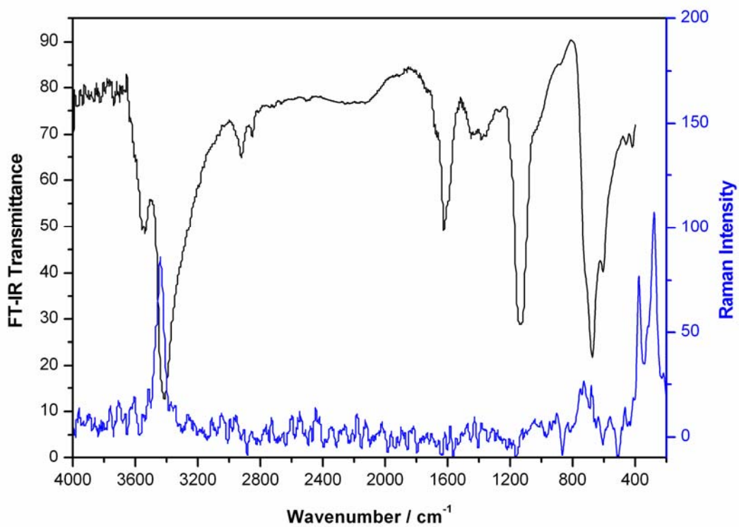
Fig. S1 IR (black) and Raman (blue) spectra of compound 1.
