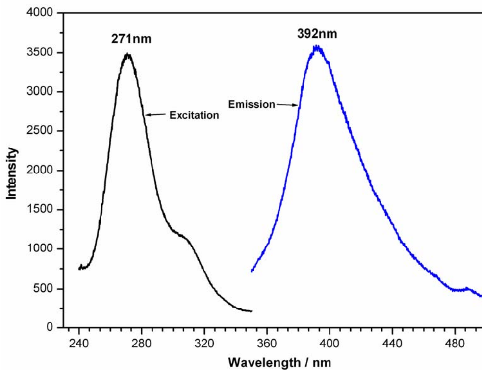
Fig. S5 Solid state emission spectra of 1.
