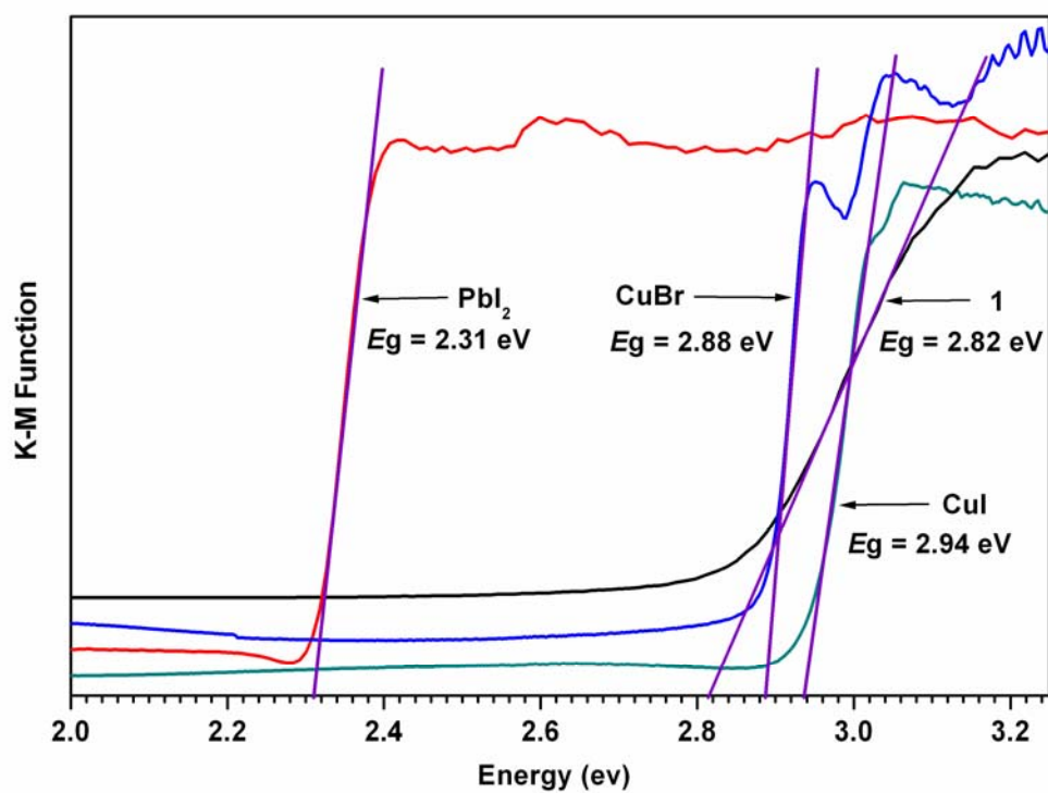
Fig. S4 Optical absorption spectra for solid samples of \text{PbI}_2 , \text{CuBr} , \text{CuI} and 1.
