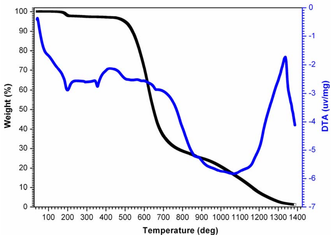
Fig. S2 TG/DTA curves of compound 1.
